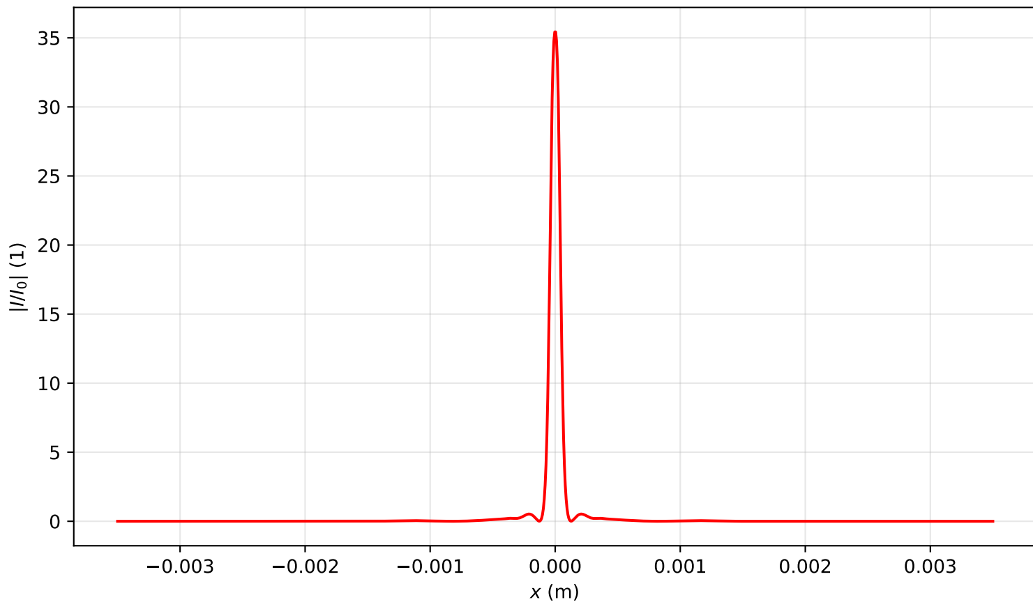
Intensity profile I(x, y = 0, z = 1.672)/I_0 , P_{in}=3.0P_{cr} , artificial time
